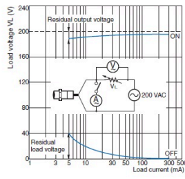
E2E-X□Y□ at 200 VAC
