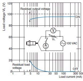
E2E-X□Y□ at 100 VAC
