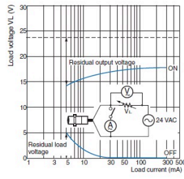
E2E-X□Y□ at 24 VAC
